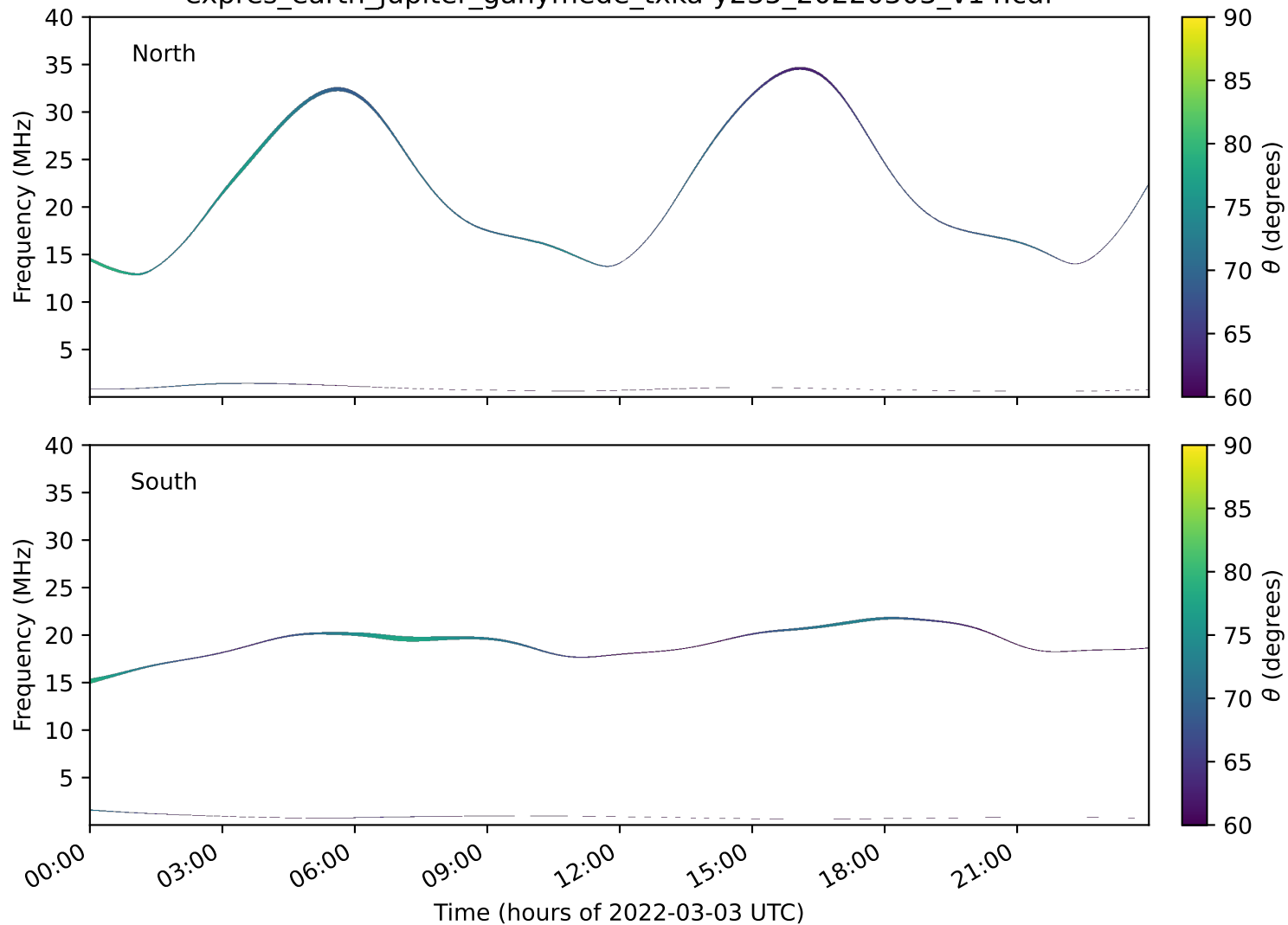
expres_earth_jupiter_ganymede_txka-y235_20220303_v14.cdf
