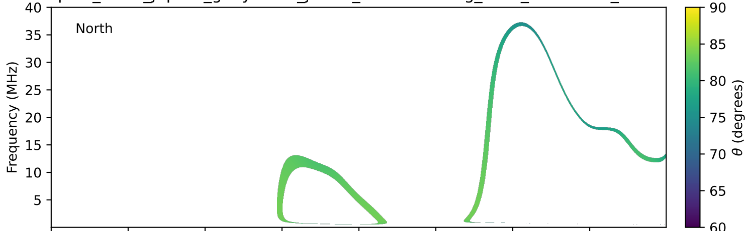
expres_earth_jupiter_ganymede_jrm33_lossc-wid1deg_3kev_20220331_v11.cdf
