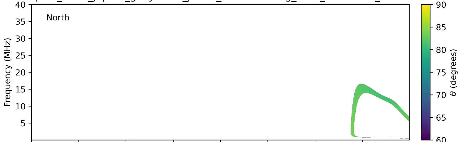
expres_earth_jupiter_ganymede_jrm33_lossc-wid1deg_3kev_20220309_v11.cdf
