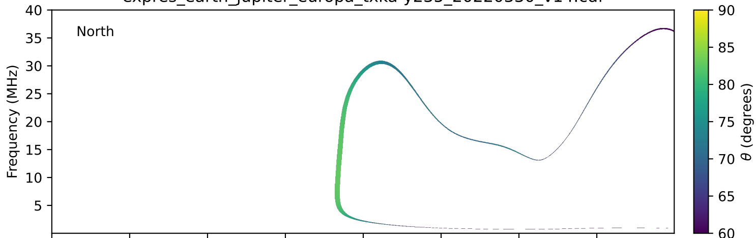
expres_earth_jupiter_europa_txka-y235_20220330_v14.cdf
