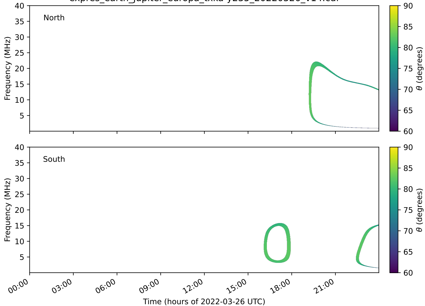
expres_earth_jupiter_europa_txka-y235_20220326_v14.cdf
