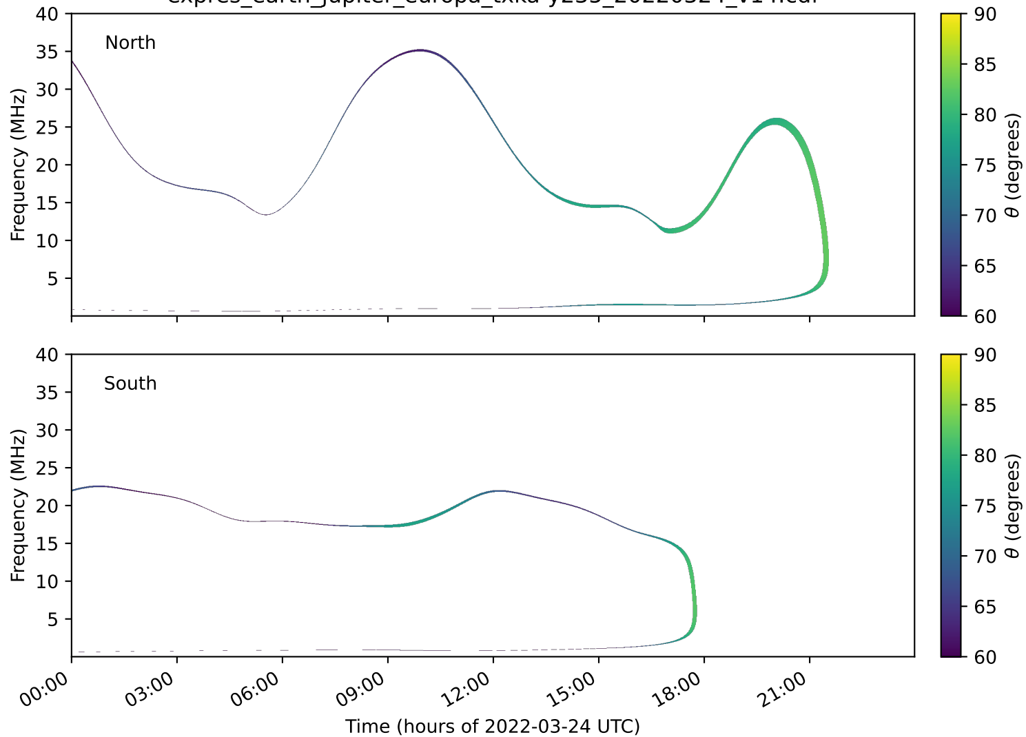
expres_earth_jupiter_europa_txka-y235_20220324_v14.cdf
