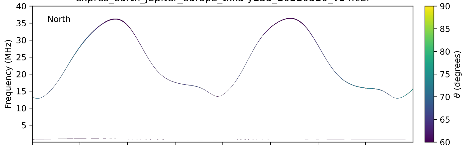
expres_earth_jupiter_europa_txka-y235_20220320_v14.cdf
