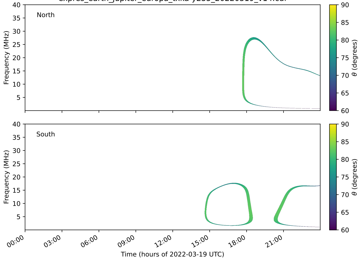
expres_earth_jupiter_europa_txka-y235_20220319_v14.cdf
