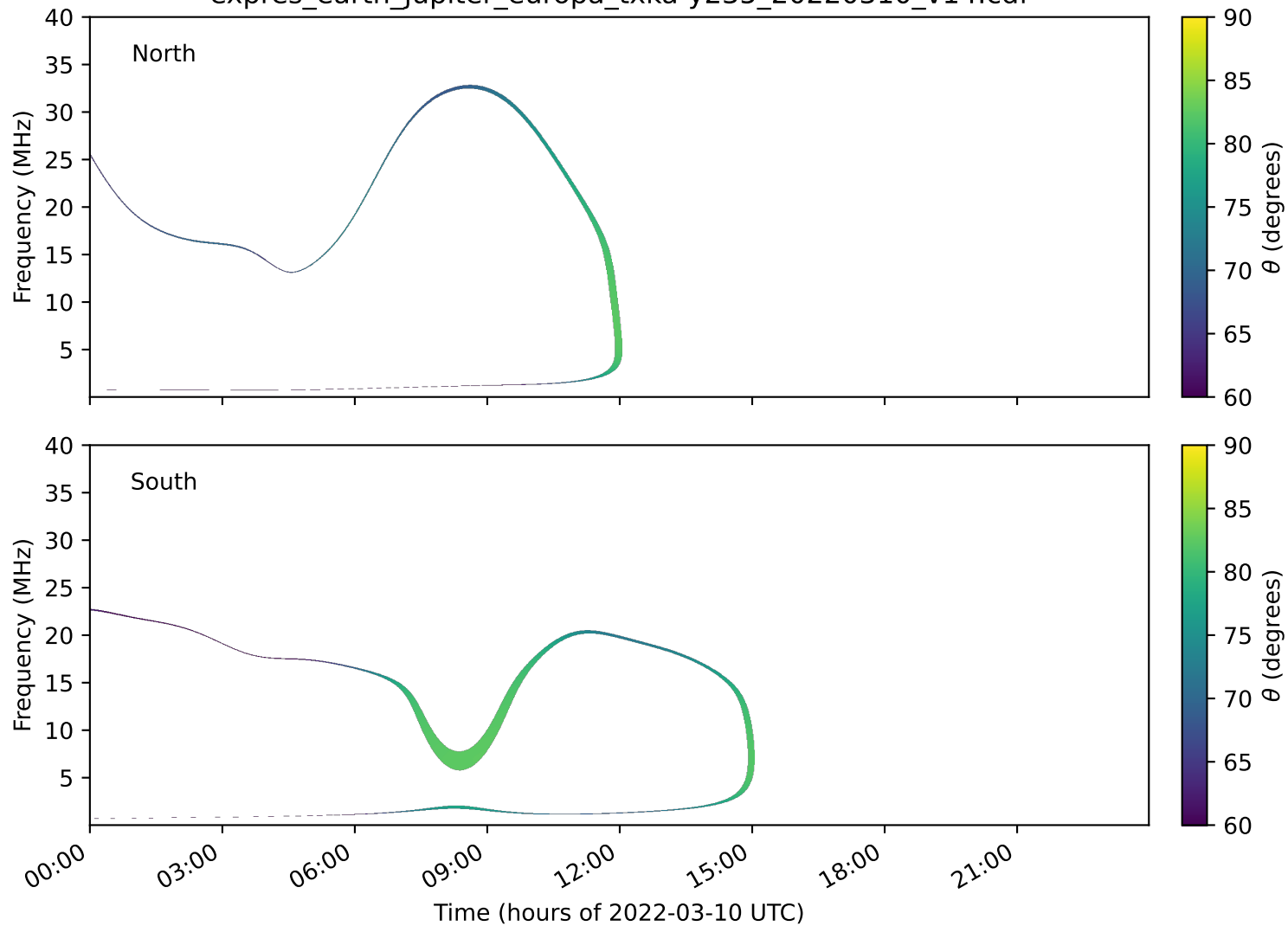
expres_earth_jupiter_europa_txka-y235_20220310_v14.cdf
