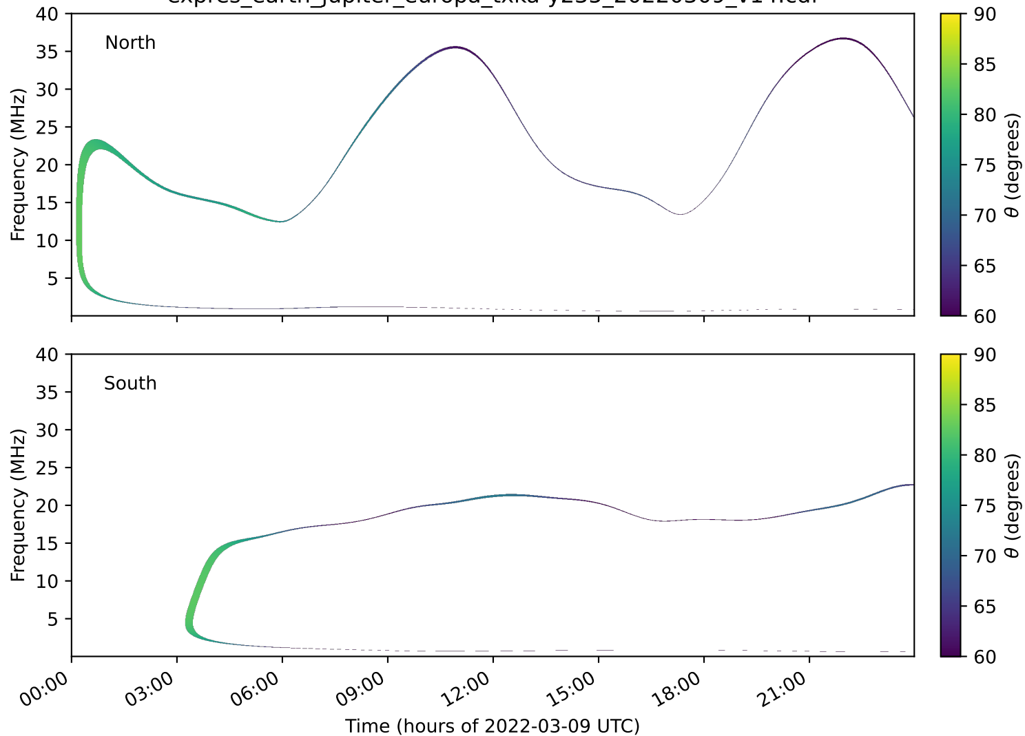
expres_earth_jupiter_europa_txka-y235_20220309_v14.cdf
