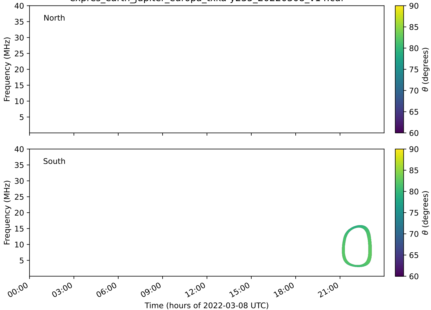
expres_earth_jupiter_europa_txka-y235_20220308_v14.cdf
