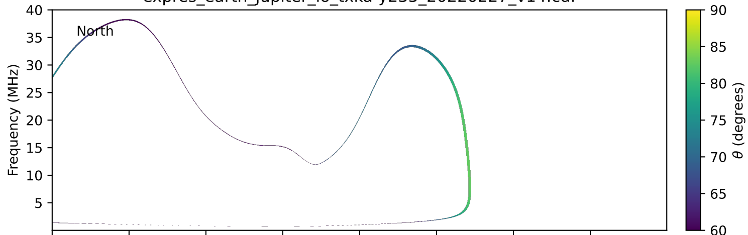
expres_earth_jupiter_io_txka-y235_20220227_v14.cdf
