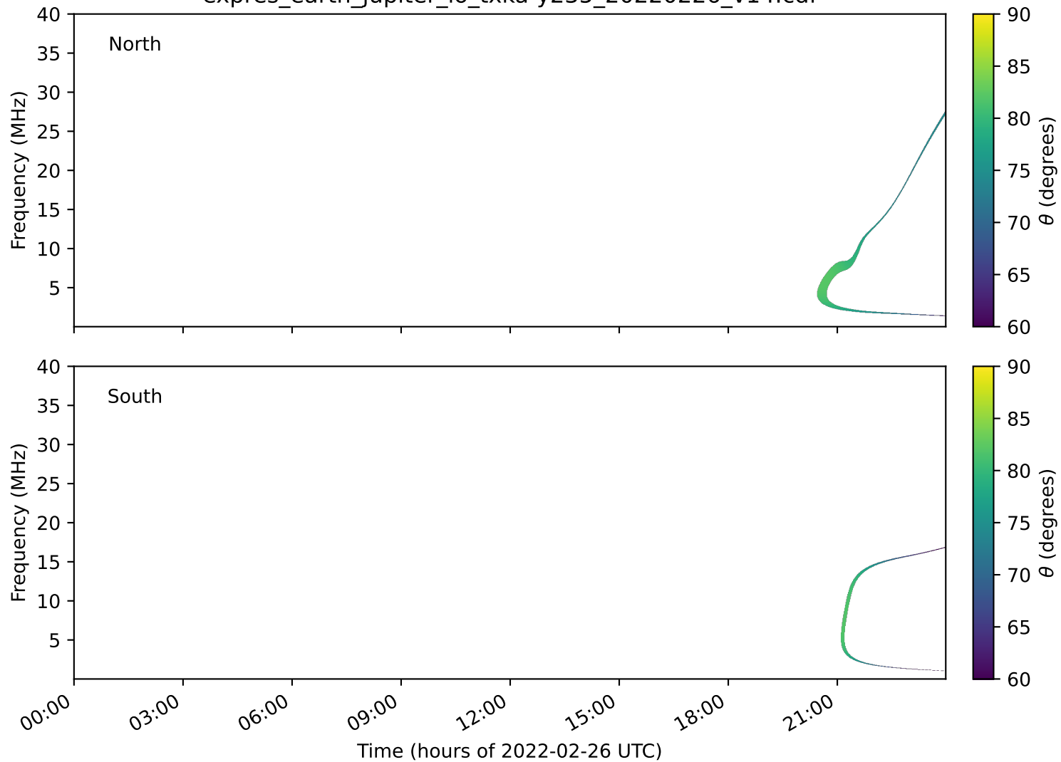
expres_earth_jupiter_io_txka-y235_20220226_v14.cdf
