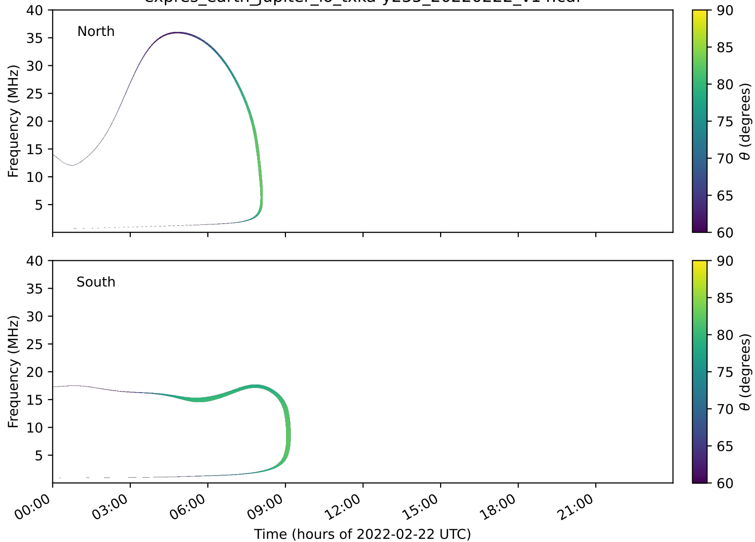
expres_earth_jupiter_io_txka-y235_20220222_v14.cdf
