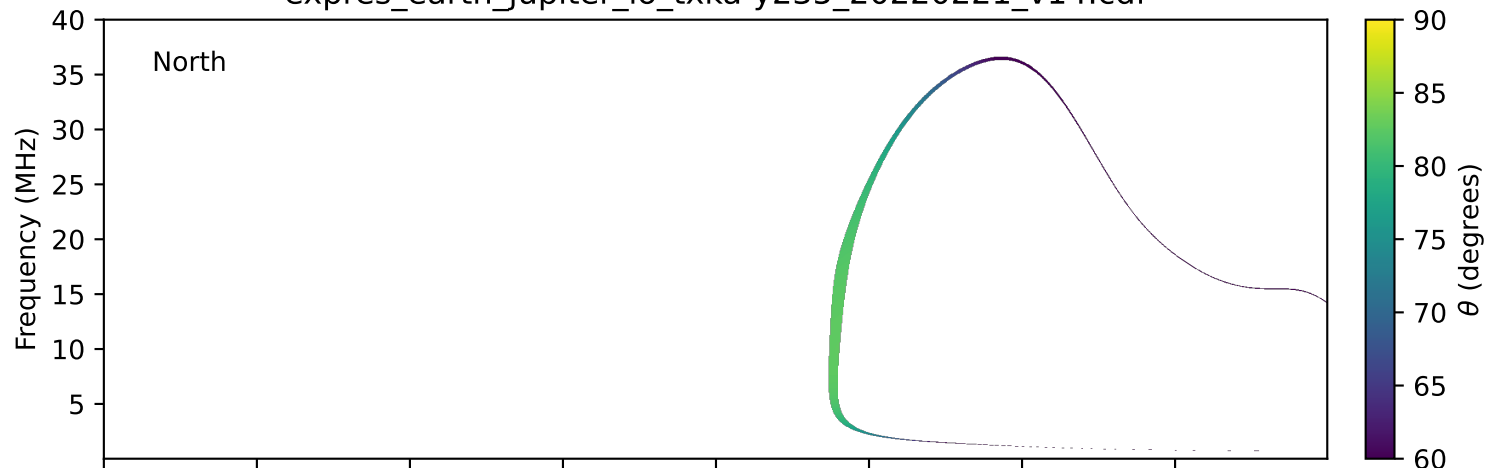
expres_earth_jupiter_io_txka-y235_20220221_v14.cdf
