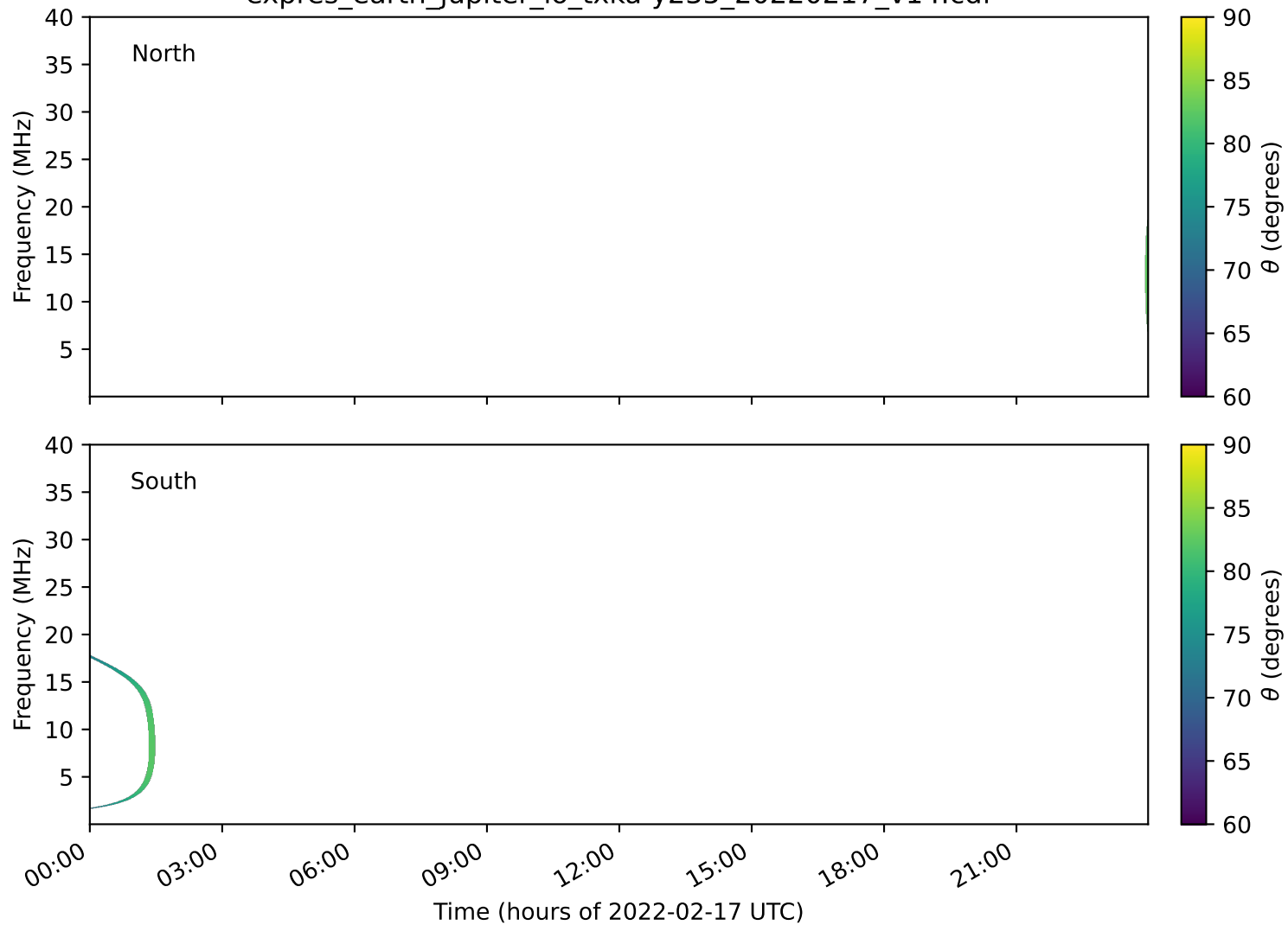
expres_earth_jupiter_io_txka-y235_20220217_v14.cdf
