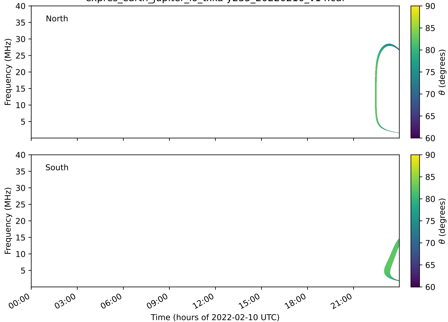
expres_earth_jupiter_io_txka-y235_20220210_v14.cdf
