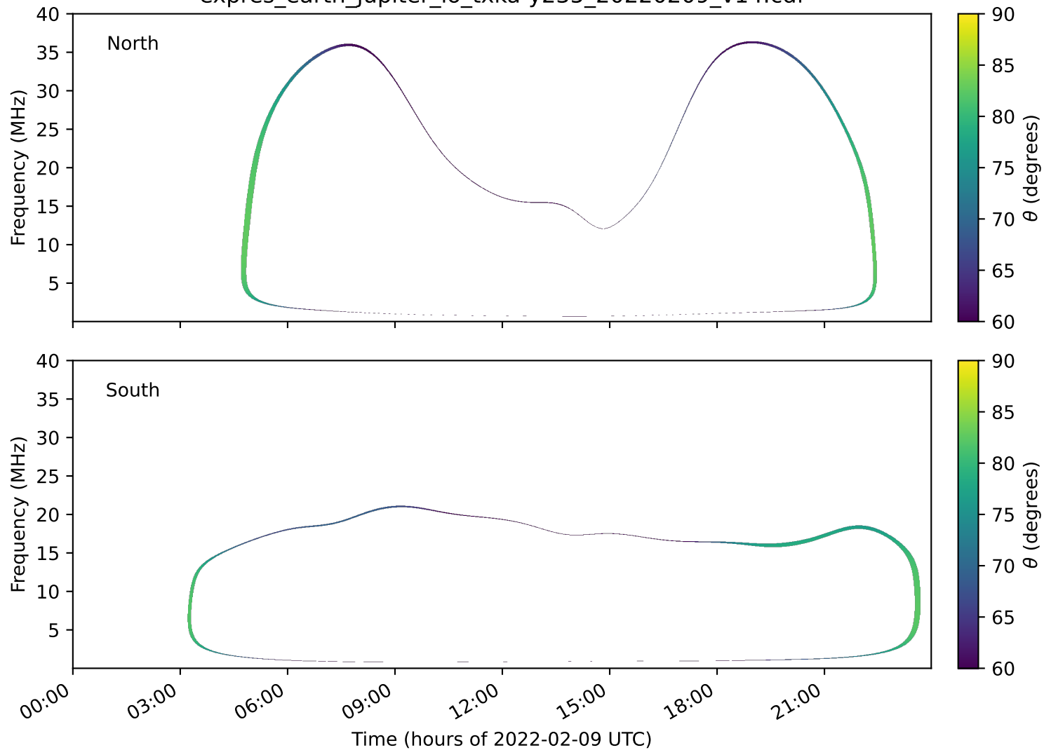
expres_earth_jupiter_io_txka-y235_20220209_v14.cdf
