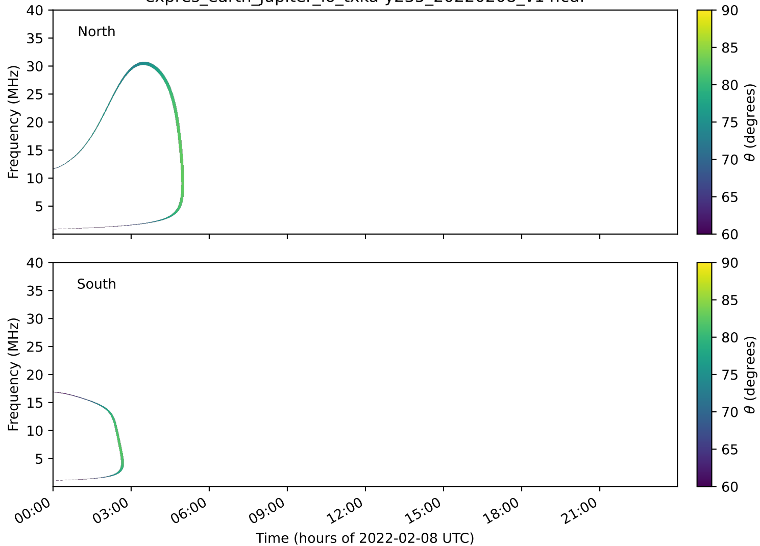
expres_earth_jupiter_io_txka-y235_20220208_v14.cdf
