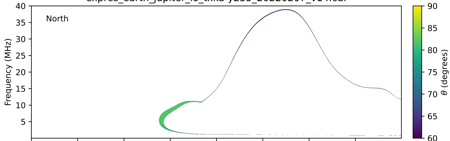
expres_earth_jupiter_io_txka-y235_20220207_v14.cdf
