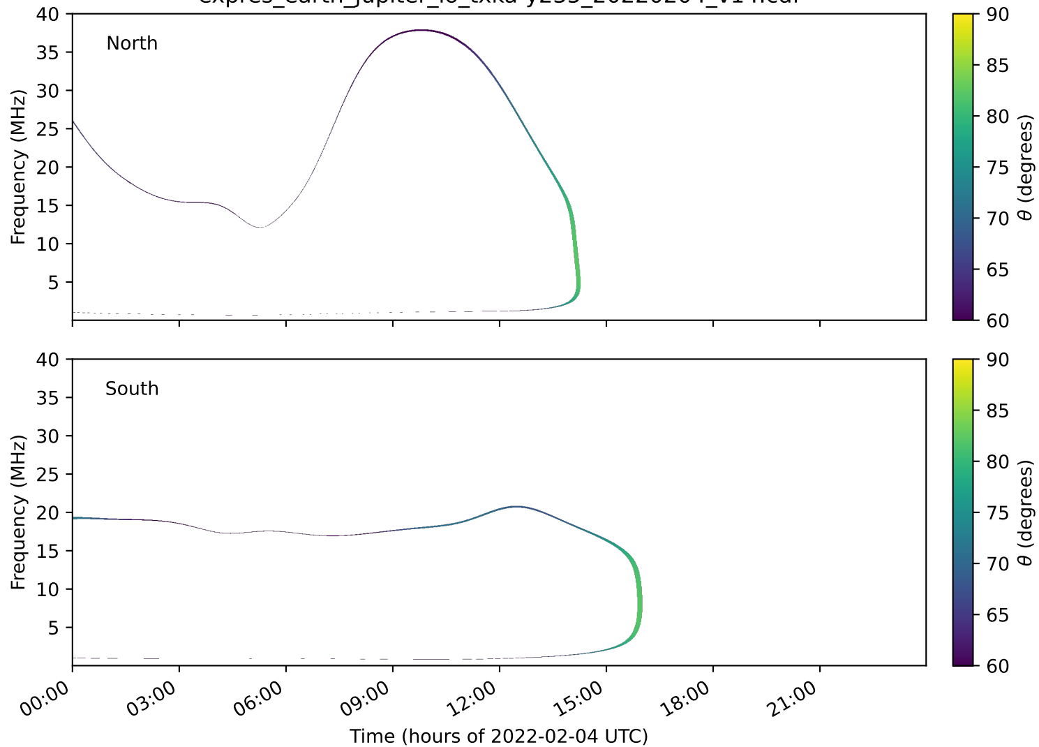
expres_earth_jupiter_io_txka-y235_20220204_v14.cdf
