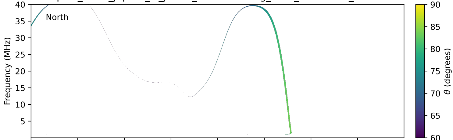
expres_earth_jupiter_io_jrm33_lossc-wid1deg_3kev_20220227_v11.cdf
