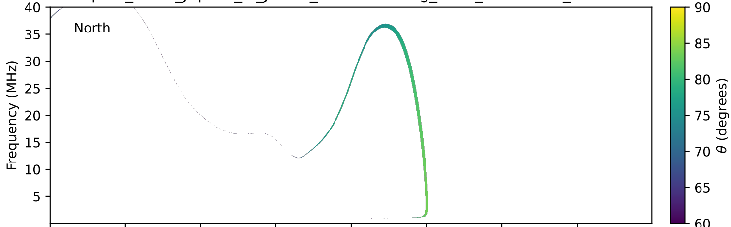
expres_earth_jupiter_io_jrm33_lossc-wid1deg_3kev_20220220_v11.cdf
