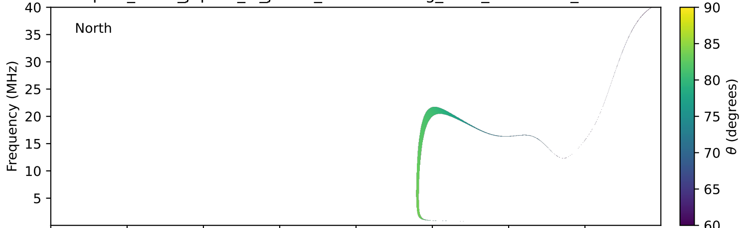
expres_earth_jupiter_io_jrm33_lossc-wid1deg_3kev_20220205_v11.cdf
