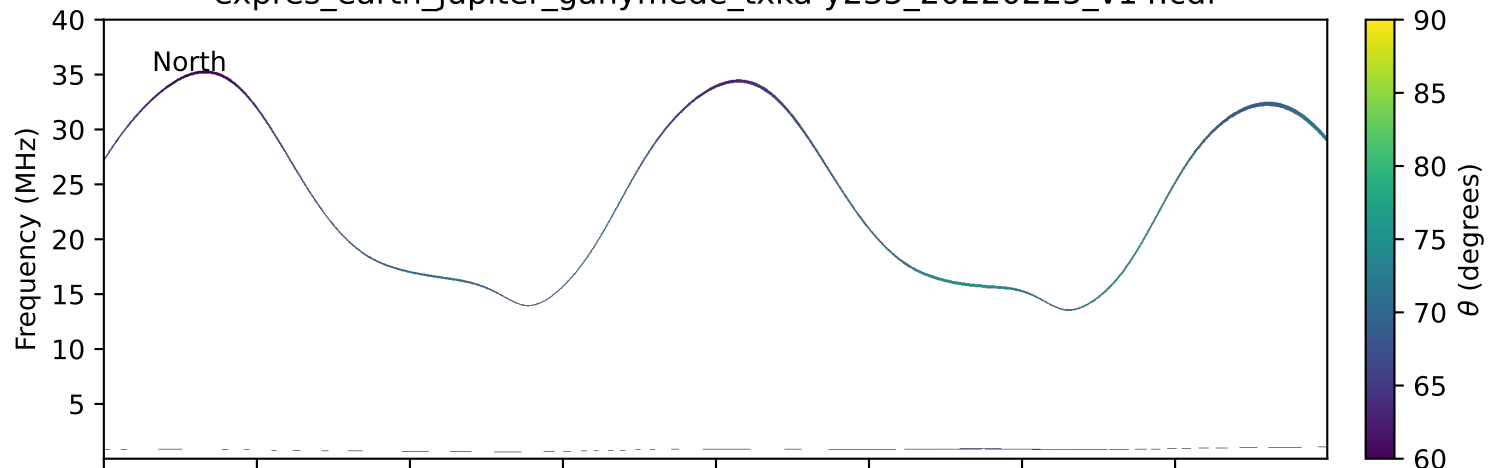
expres_earth_jupiter_ganymede_txka-y235_20220225_v14.cdf
