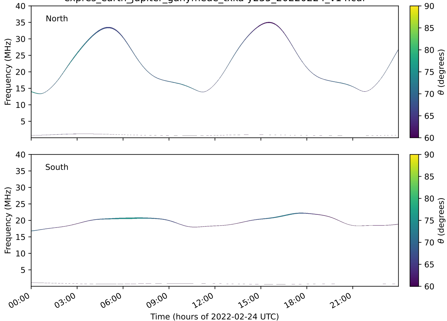
expres_earth_jupiter_ganymede_txka-y235_20220224_v14.cdf
