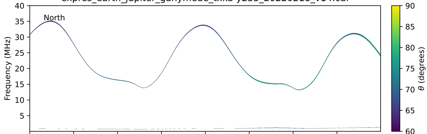
expres_earth_jupiter_ganymede_txka-y235_20220218_v14.cdf
