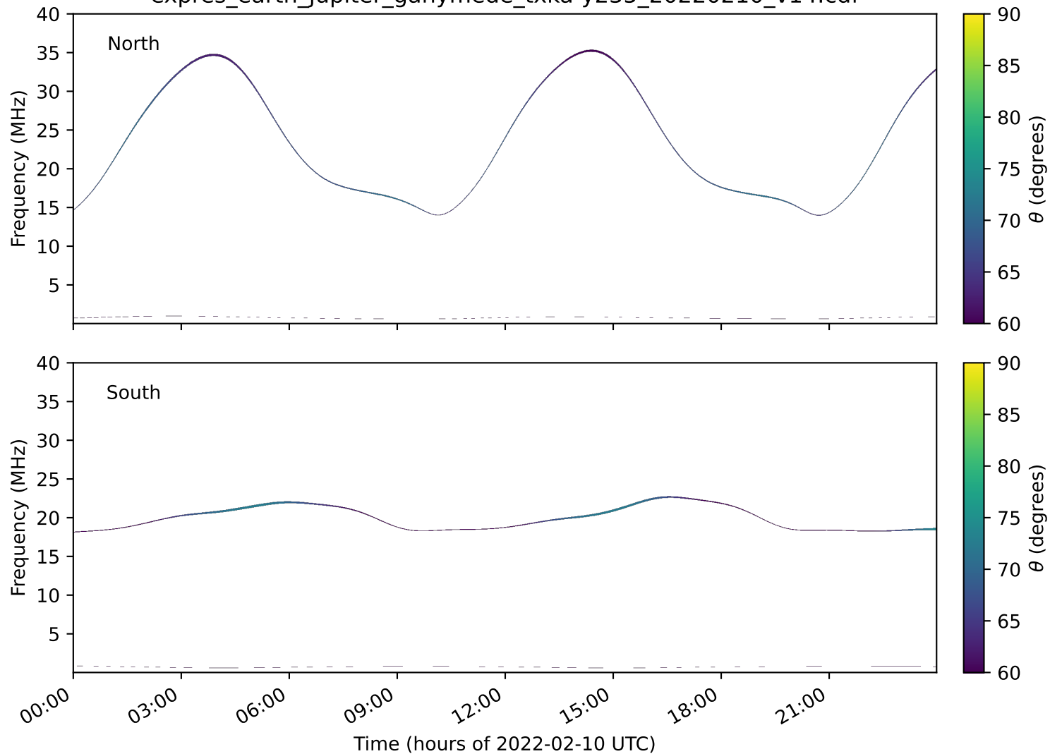
expres_earth_jupiter_ganymede_txka-y235_20220210_v14.cdf
