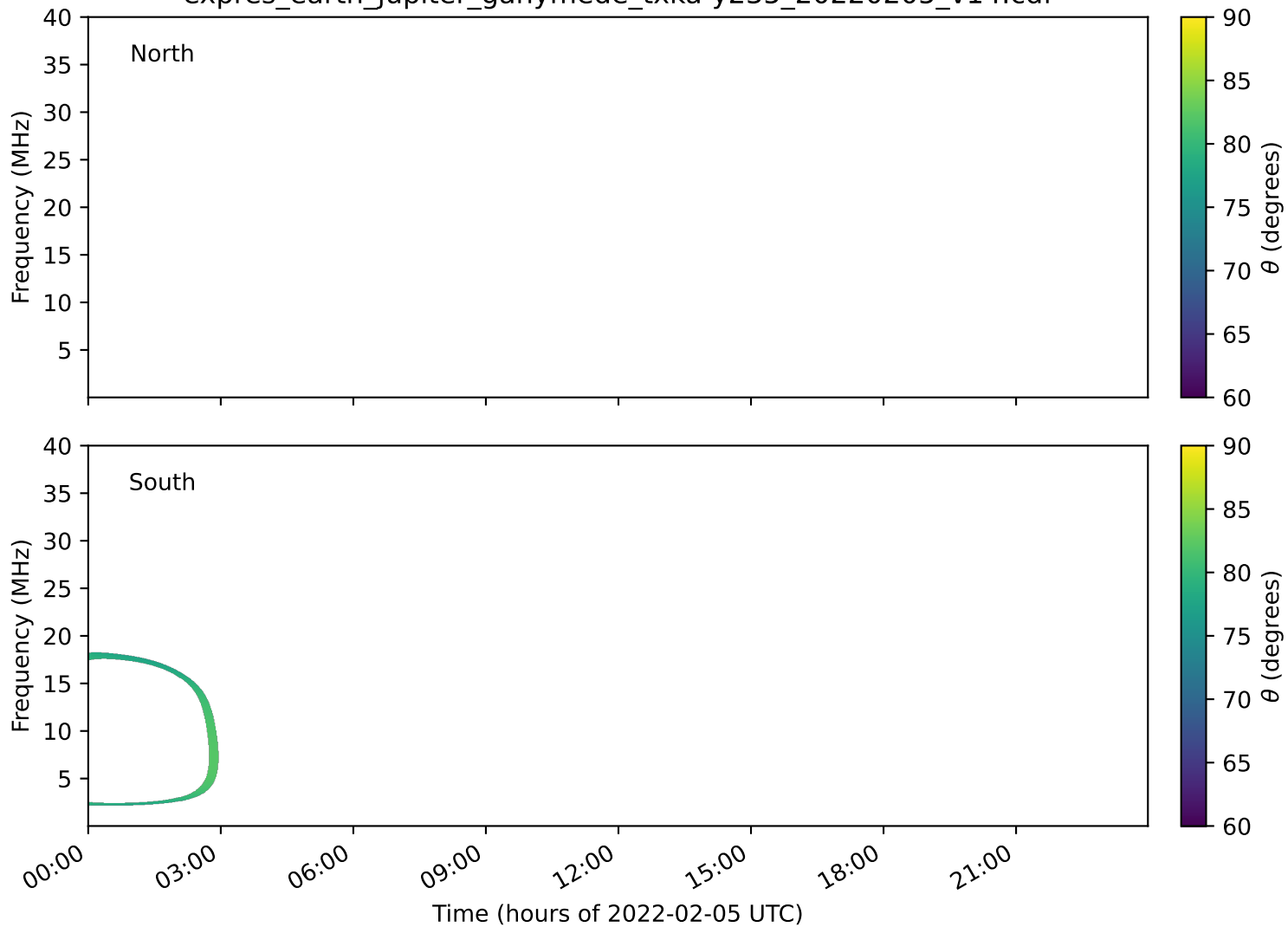
expres_earth_jupiter_ganymede_txka-y235_20220205_v14.cdf
