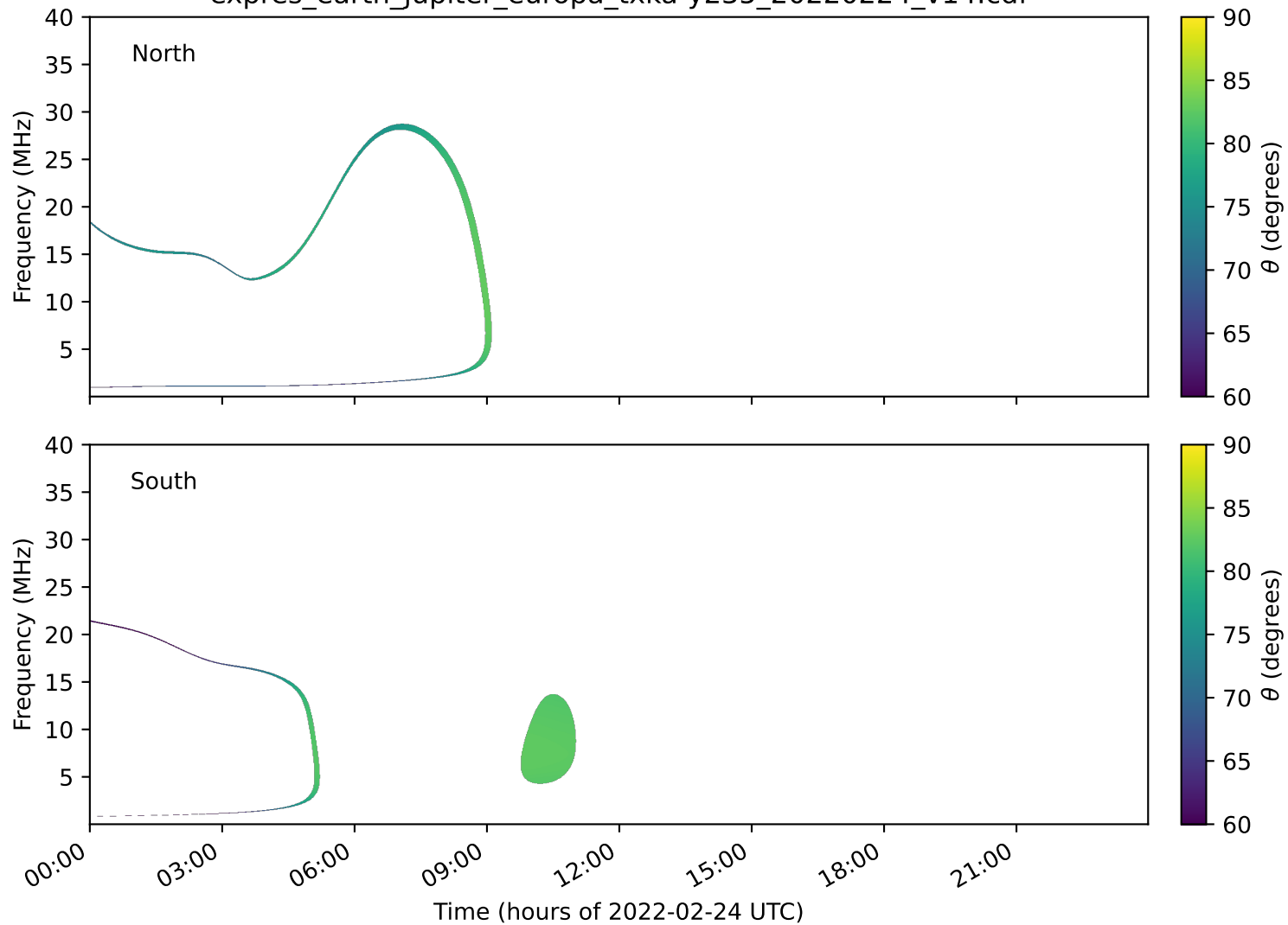
expres_earth_jupiter_europa_txka-y235_20220224_v14.cdf
