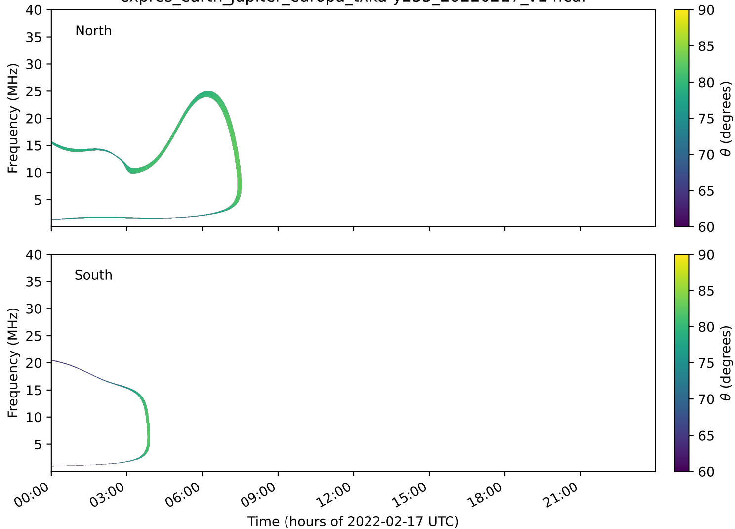
expres_earth_jupiter_europa_txka-y235_20220217_v14.cdf
