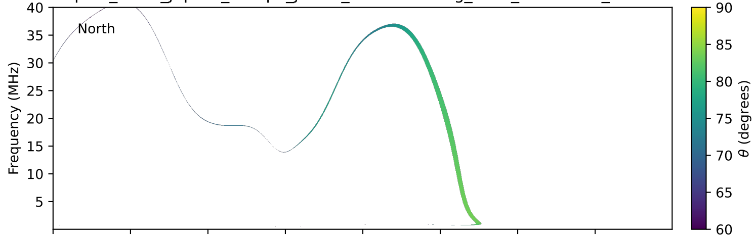
expres_earth_jupiter_europa_jrm33_lossc-wid1deg_3kev_20220213_v11.cdf
