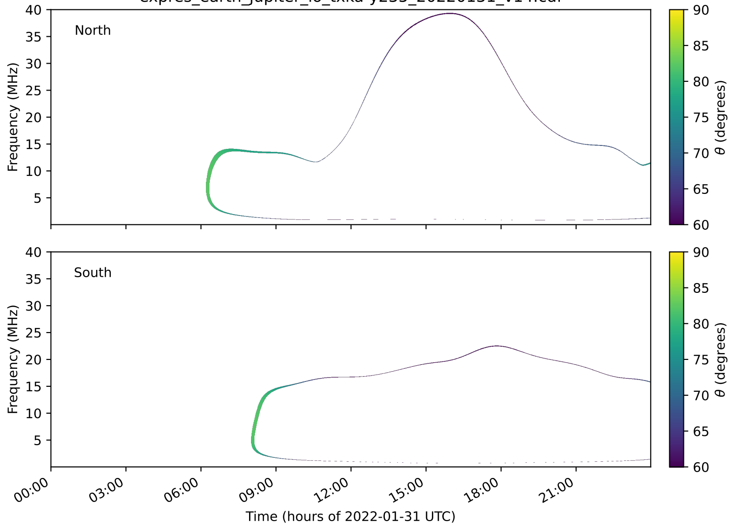
expres_earth_jupiter_io_txka-y235_20220131_v14.cdf
