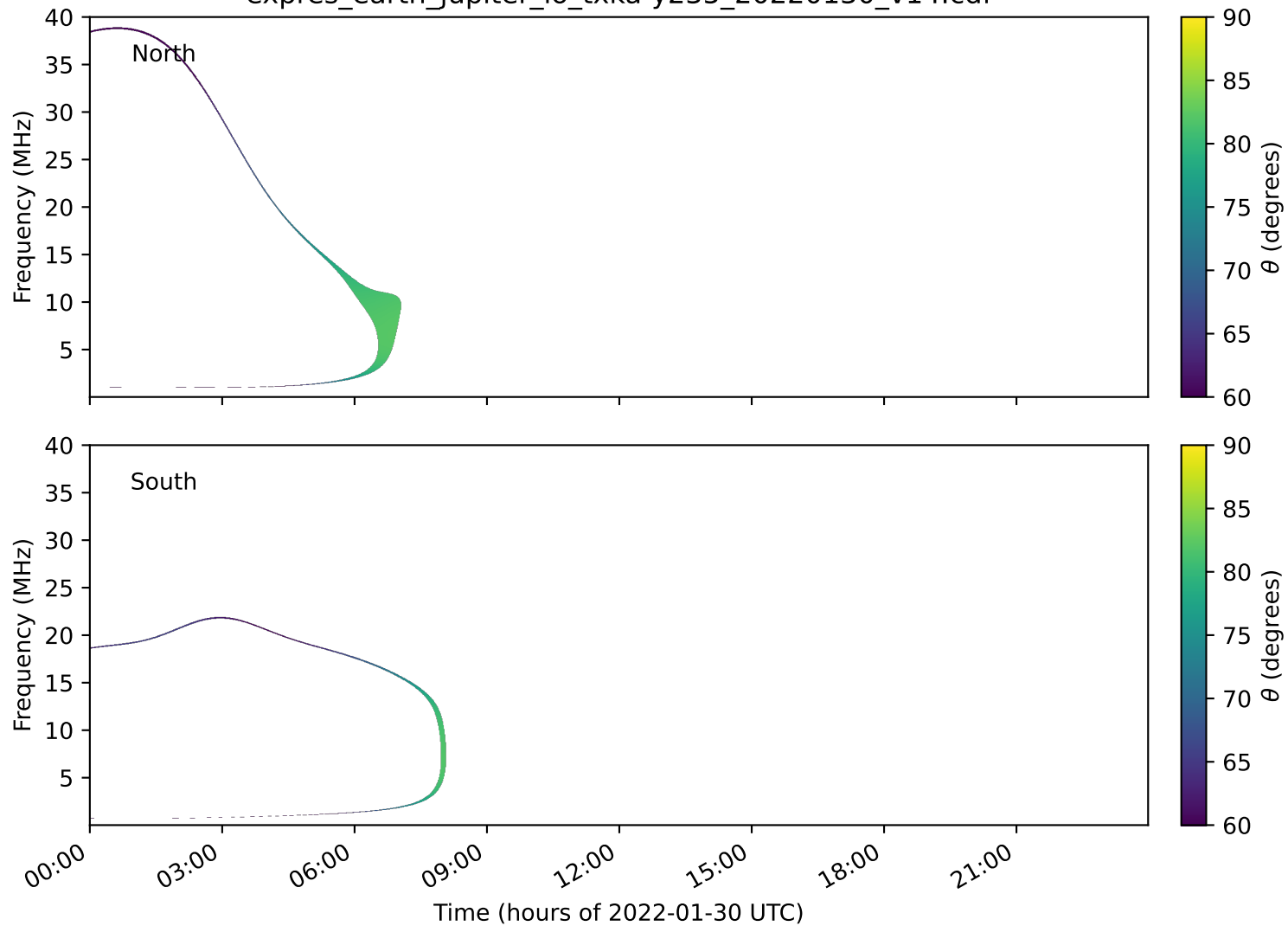
expres_earth_jupiter_io_txka-y235_20220130_v14.cdf
