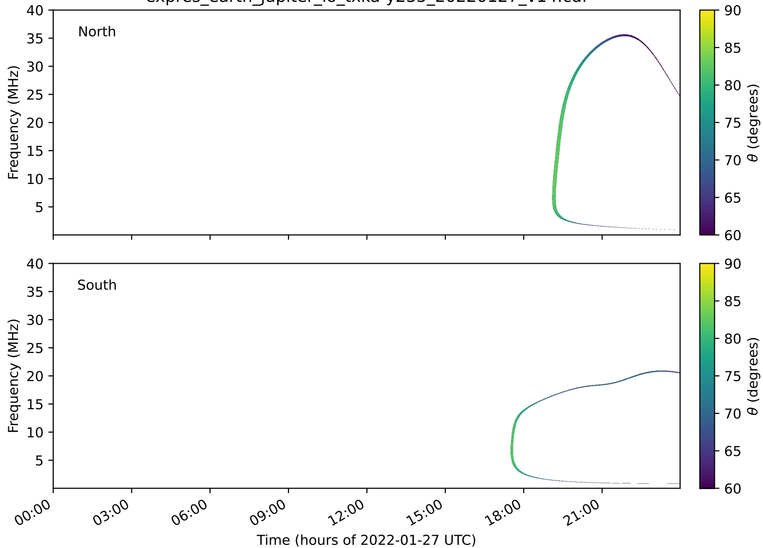
expres_earth_jupiter_io_txka-y235_20220127_v14.cdf
