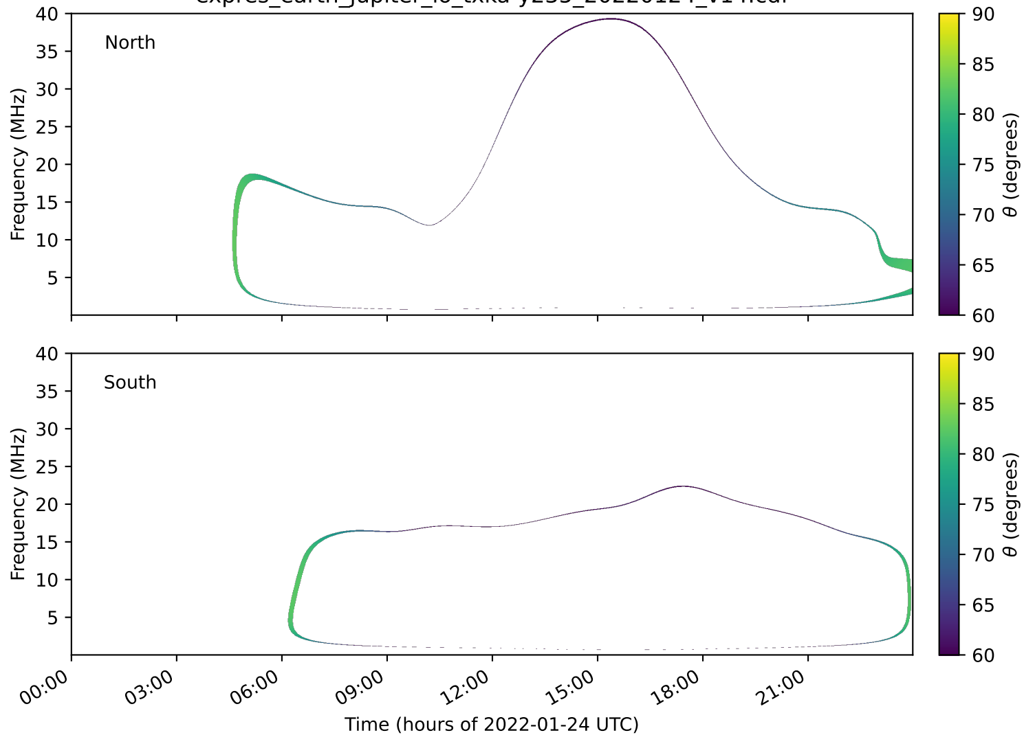
expres_earth_jupiter_io_txka-y235_20220124_v14.cdf
