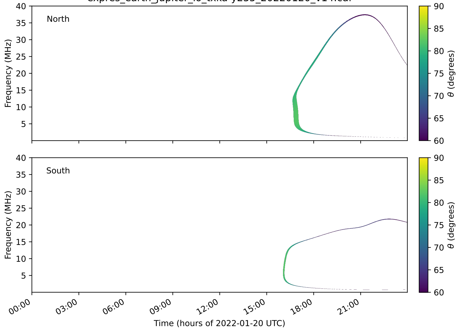
expres_earth_jupiter_io_txka-y235_20220120_v14.cdf
