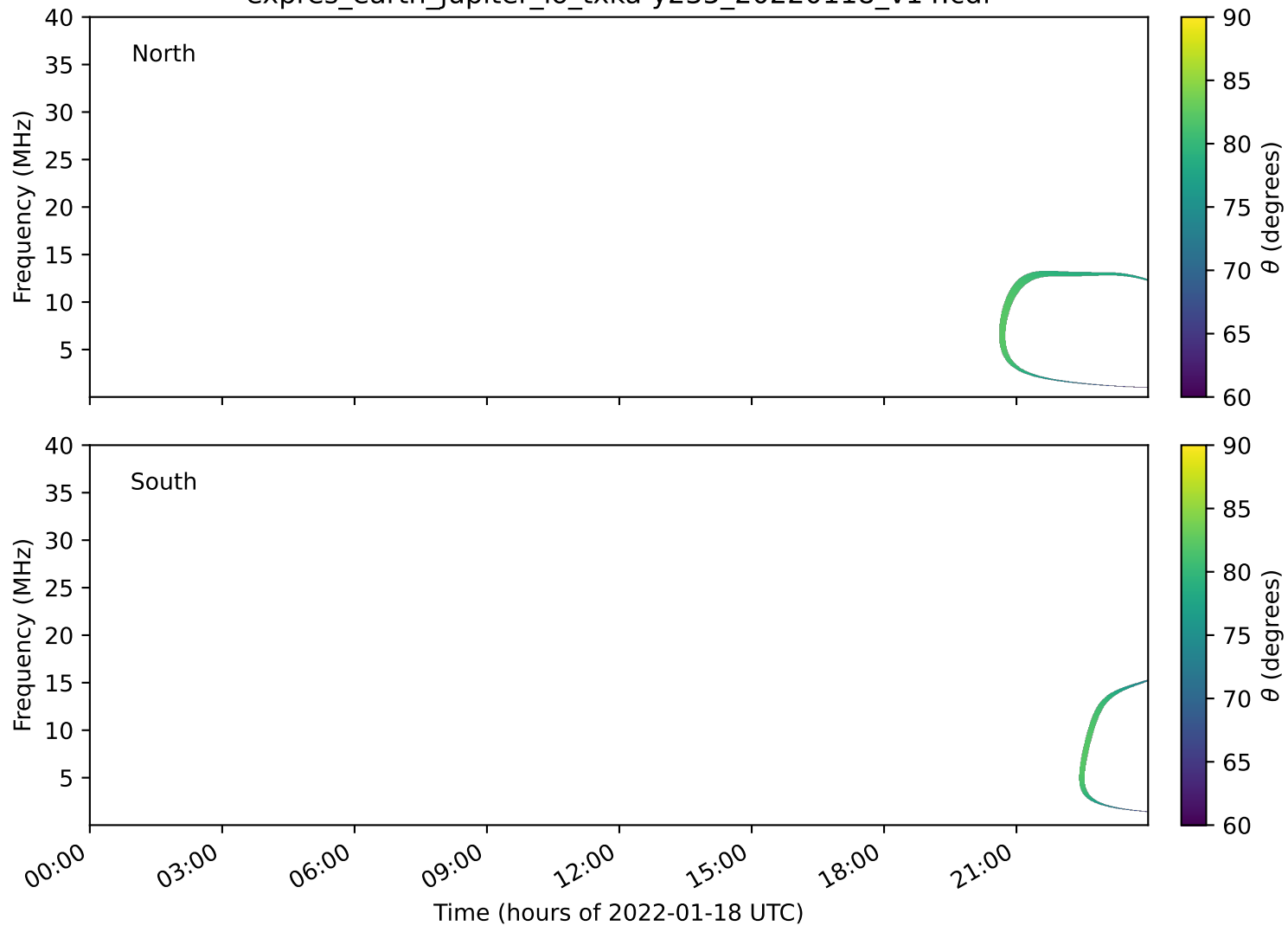
expres_earth_jupiter_io_txka-y235_20220118_v14.cdf
