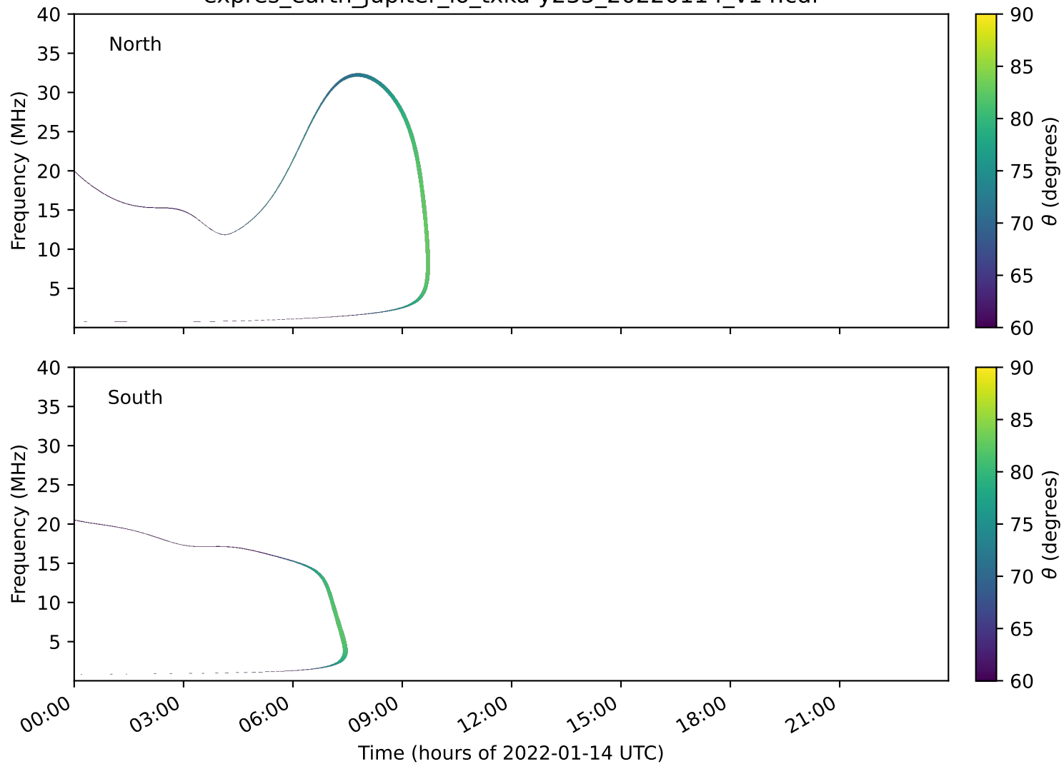
expres_earth_jupiter_io_txka-y235_20220114_v14.cdf
