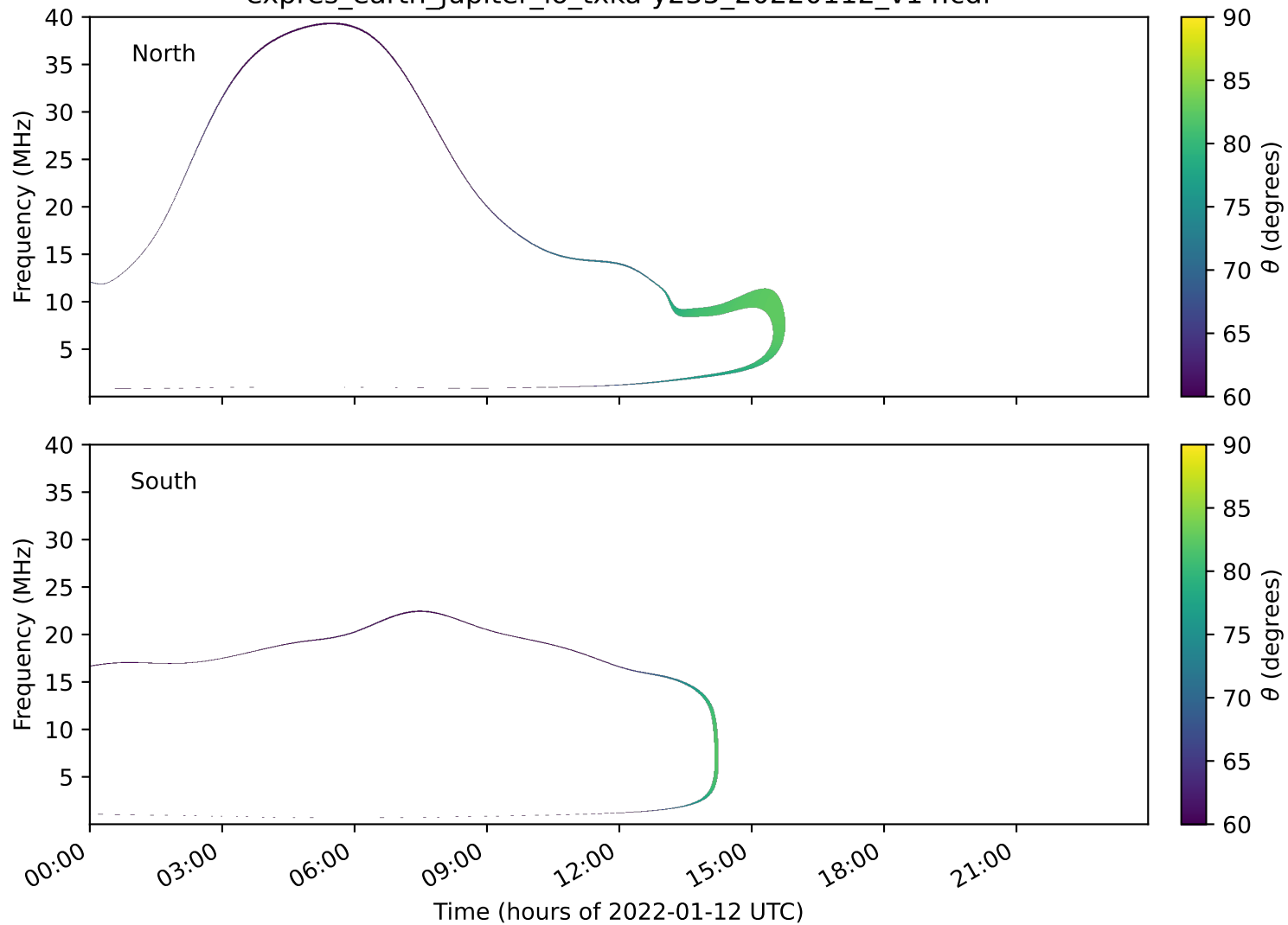
expres_earth_jupiter_io_txka-y235_20220112_v14.cdf
