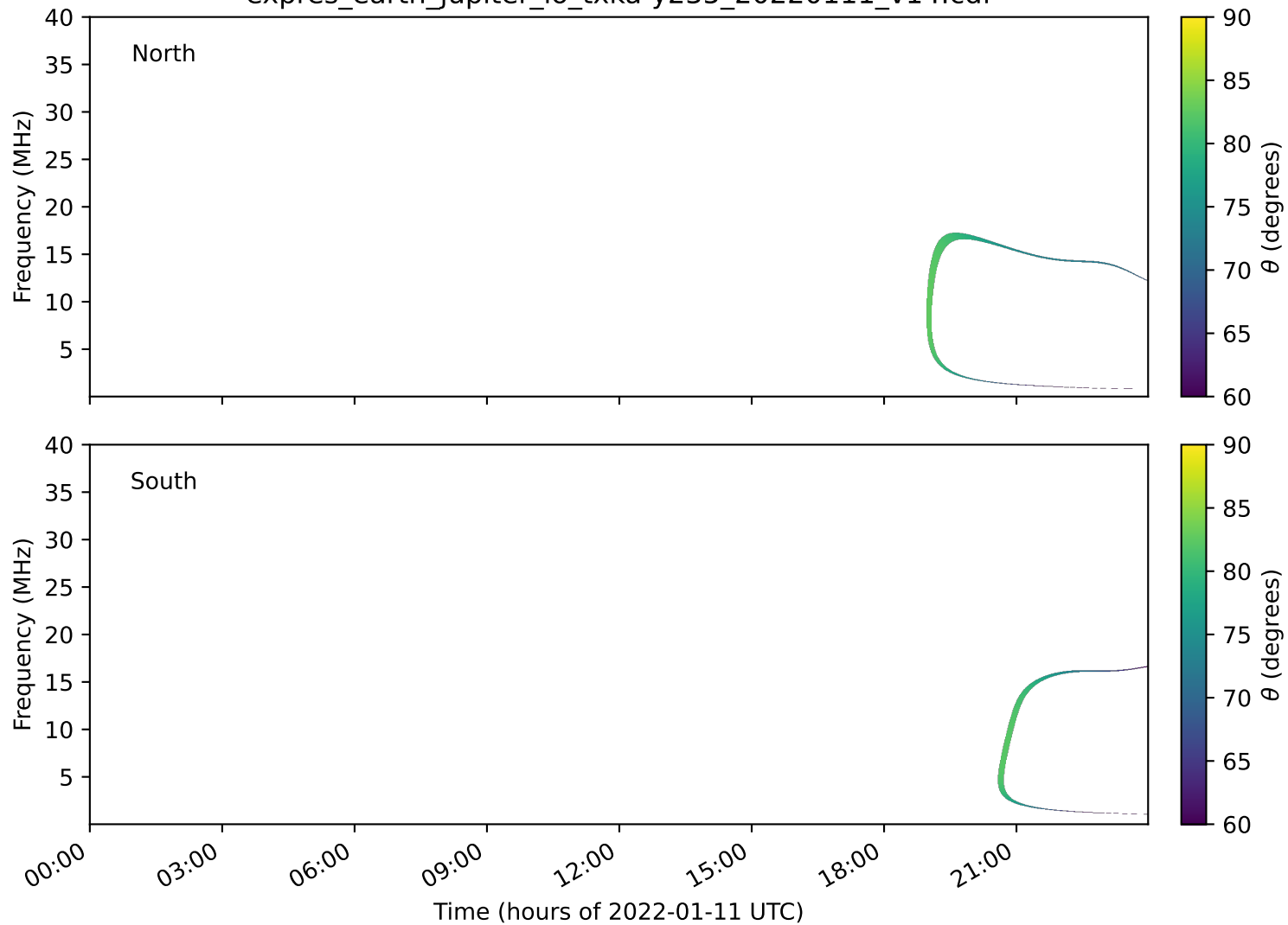
expres_earth_jupiter_io_txka-y235_20220111_v14.cdf
