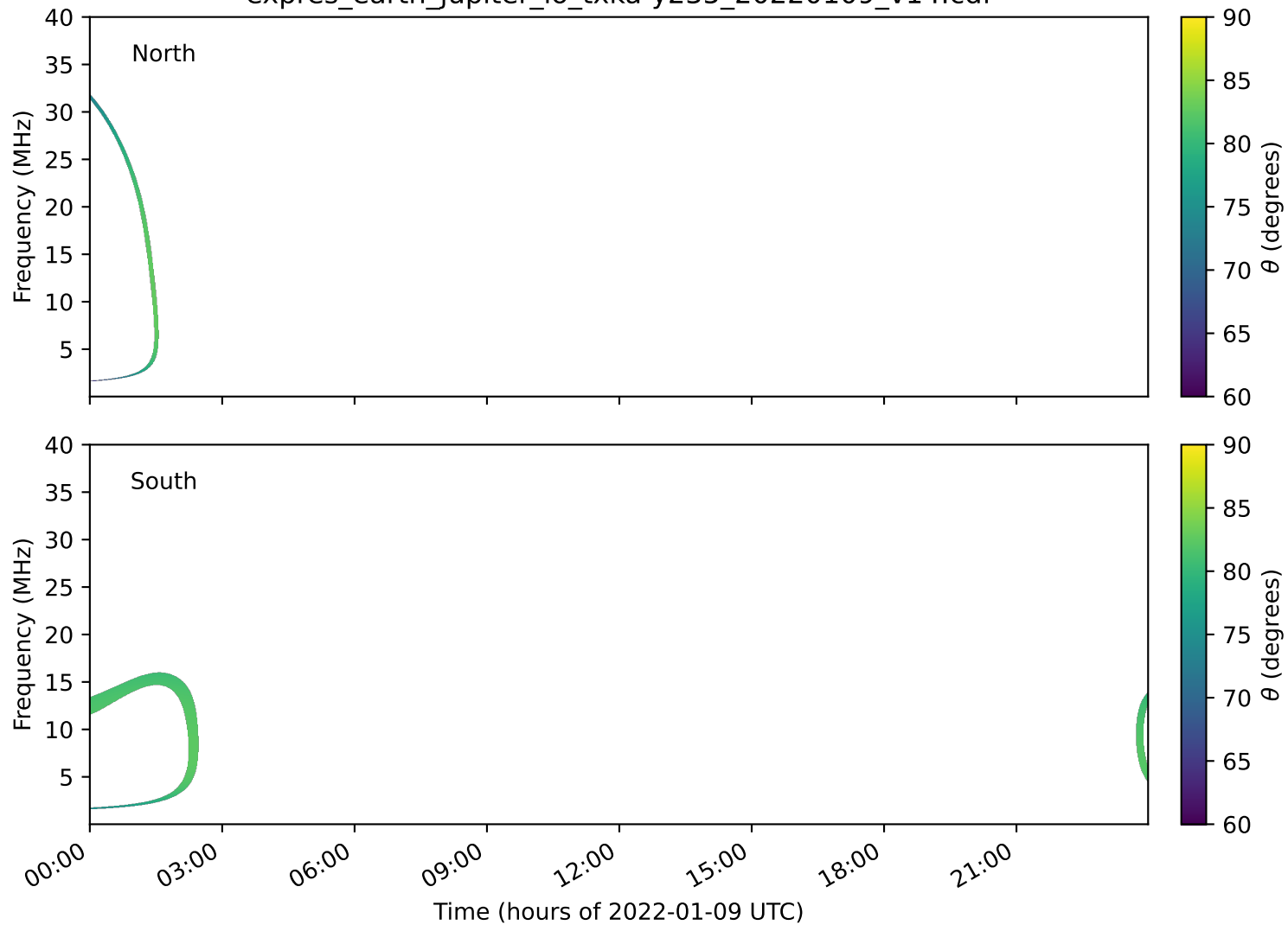
expres_earth_jupiter_io_txka-y235_20220109_v14.cdf
