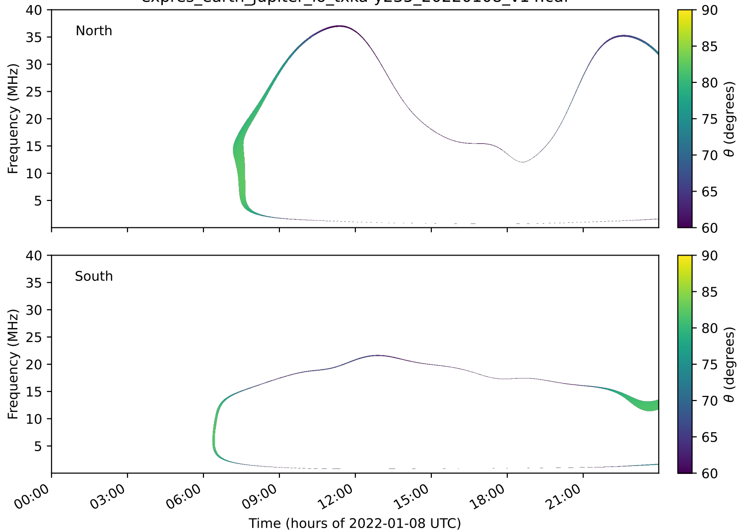
expres_earth_jupiter_io_txka-y235_20220108_v14.cdf
