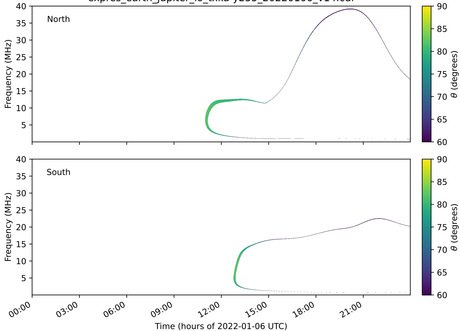
expres_earth_jupiter_io_txka-y235_20220106_v14.cdf
