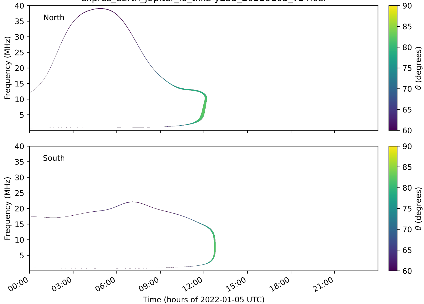
expres_earth_jupiter_io_txka-y235_20220105_v14.cdf
