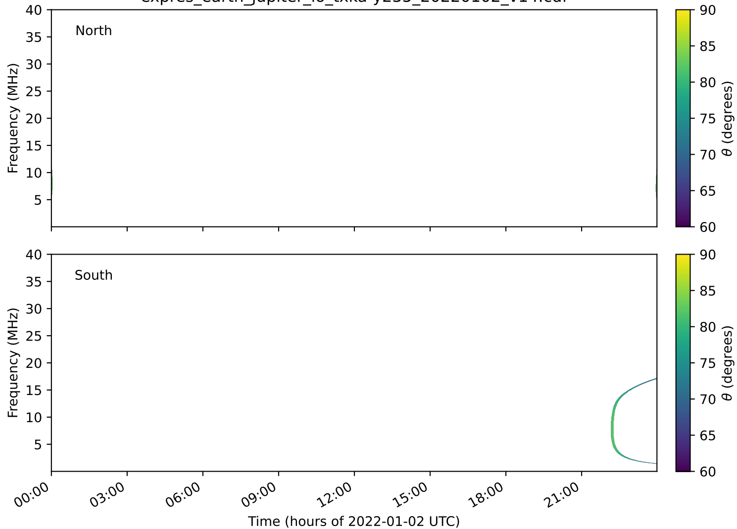
expres_earth_jupiter_io_txka-y235_20220102_v14.cdf
