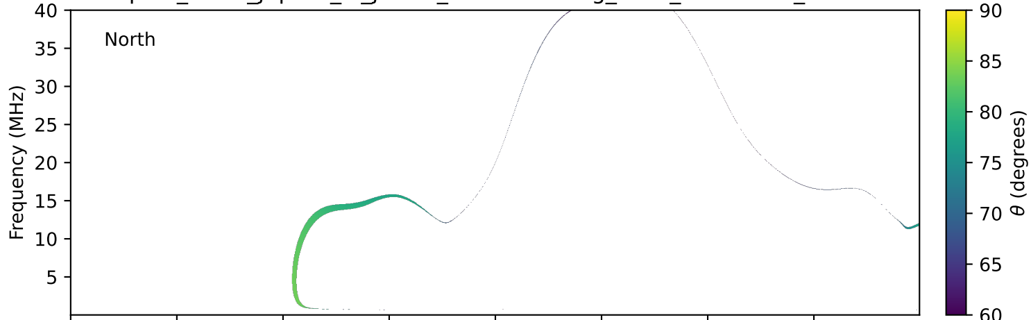
expres_earth_jupiter_io_jrm33_lossc-wid1deg_3kev_20220131_v11.cdf
