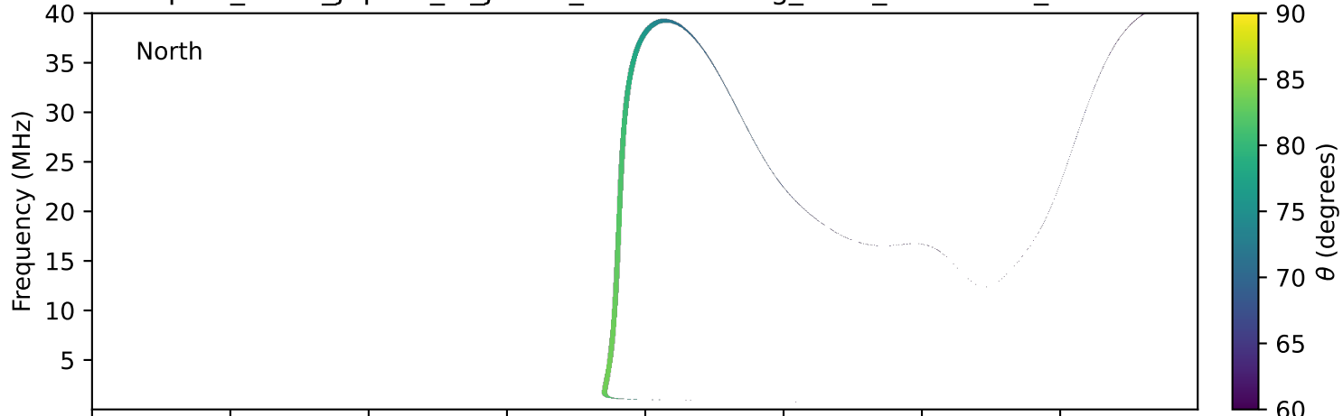
expres_earth_jupiter_io_jrm33_lossc-wid1deg_3kev_20220122_v11.cdf
