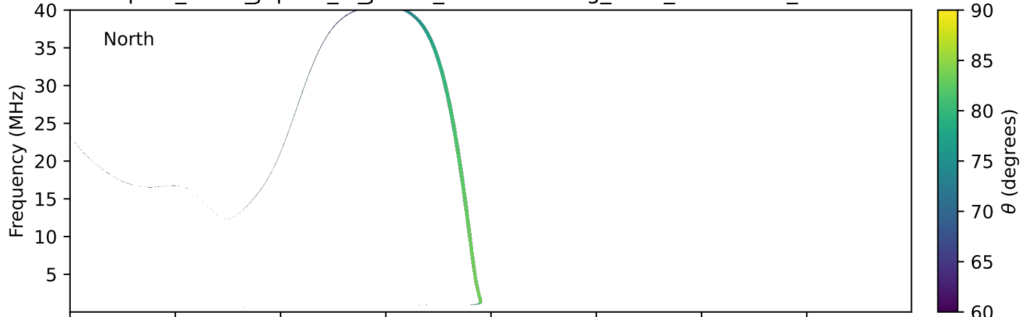
expres_earth_jupiter_io_jrm33_lossc-wid1deg_3kev_20220121_v11.cdf
