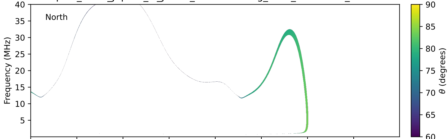
expres_earth_jupiter_io_jrm33_lossc-wid1deg_3kev_20220119_v11.cdf
